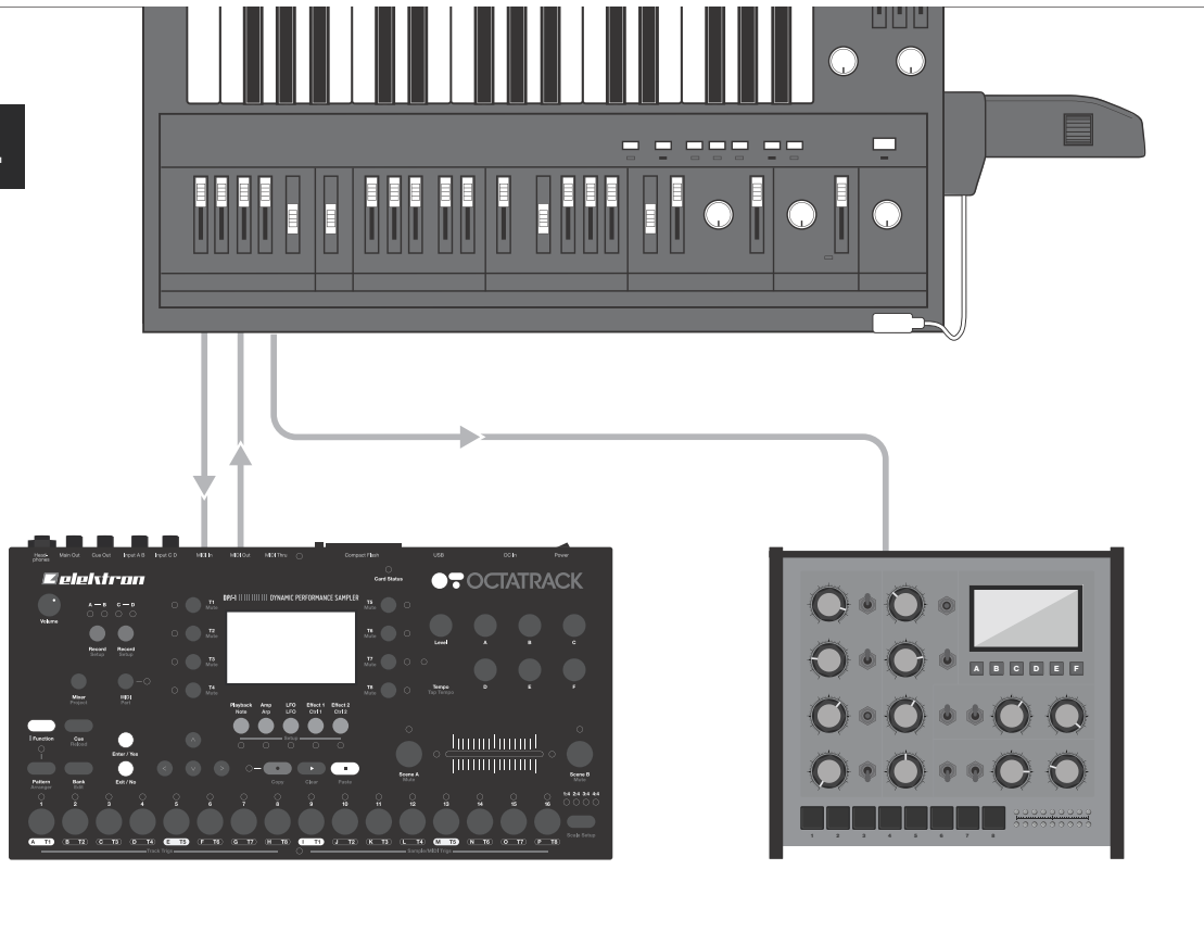
Fig 5. The MIDI OUT of an external synthesizer is connected to the Octatrack MIDI IN. The Octatrack MIDI OUT is connected to the MIDI IN of the synthesizer. A synth module is connected to the MIDI THRU of the synthesizer. The Octatrack can MIDI control both the synthesizer and the synth module. At the same time the keyboard of the synthesizer can be used to play Octatrack samples, play the synthesizer itself as well as the synth module.
